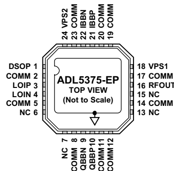
Figure 2. Pin Configuration
