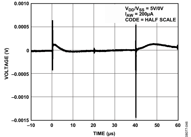
Figure 35. Digital Feedthrough
