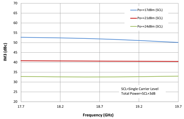
IM3 versus Frequency
