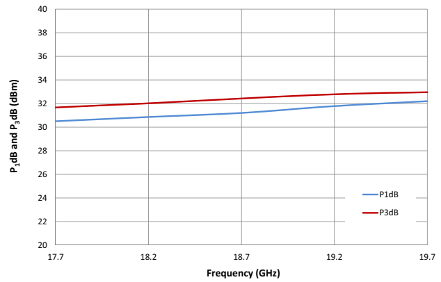
P 1 dB and P 3 dB versus Frequency (Vd=5V)
