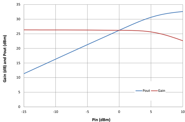
Gain and Pout versus Pin (Vd=5V and 18.7GHz)
