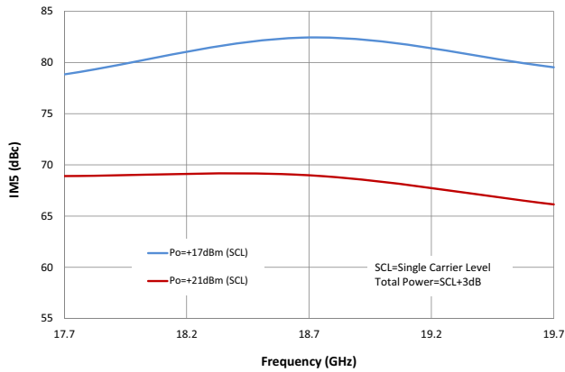
IM5 versus Frequency
