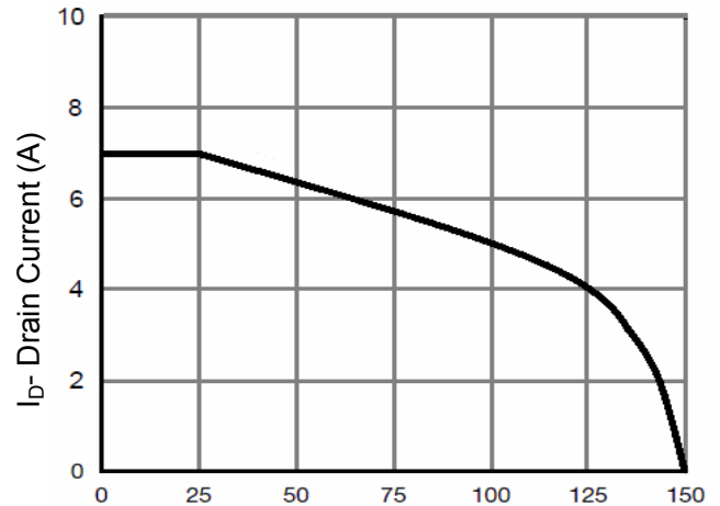
Figure 10 Current De-rating
