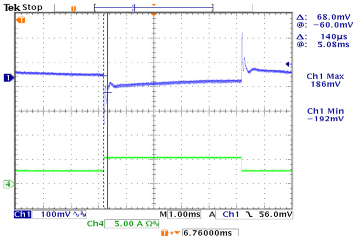
50%~100% Load Transient(AC) at 25°C@115V
