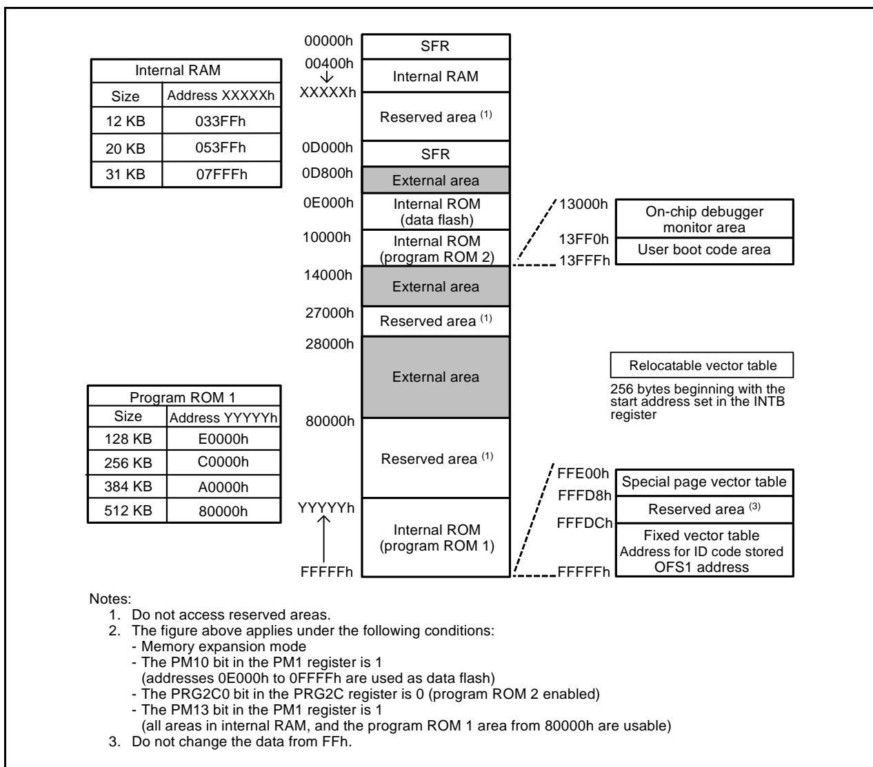
Figure 3.2 Memory Map
