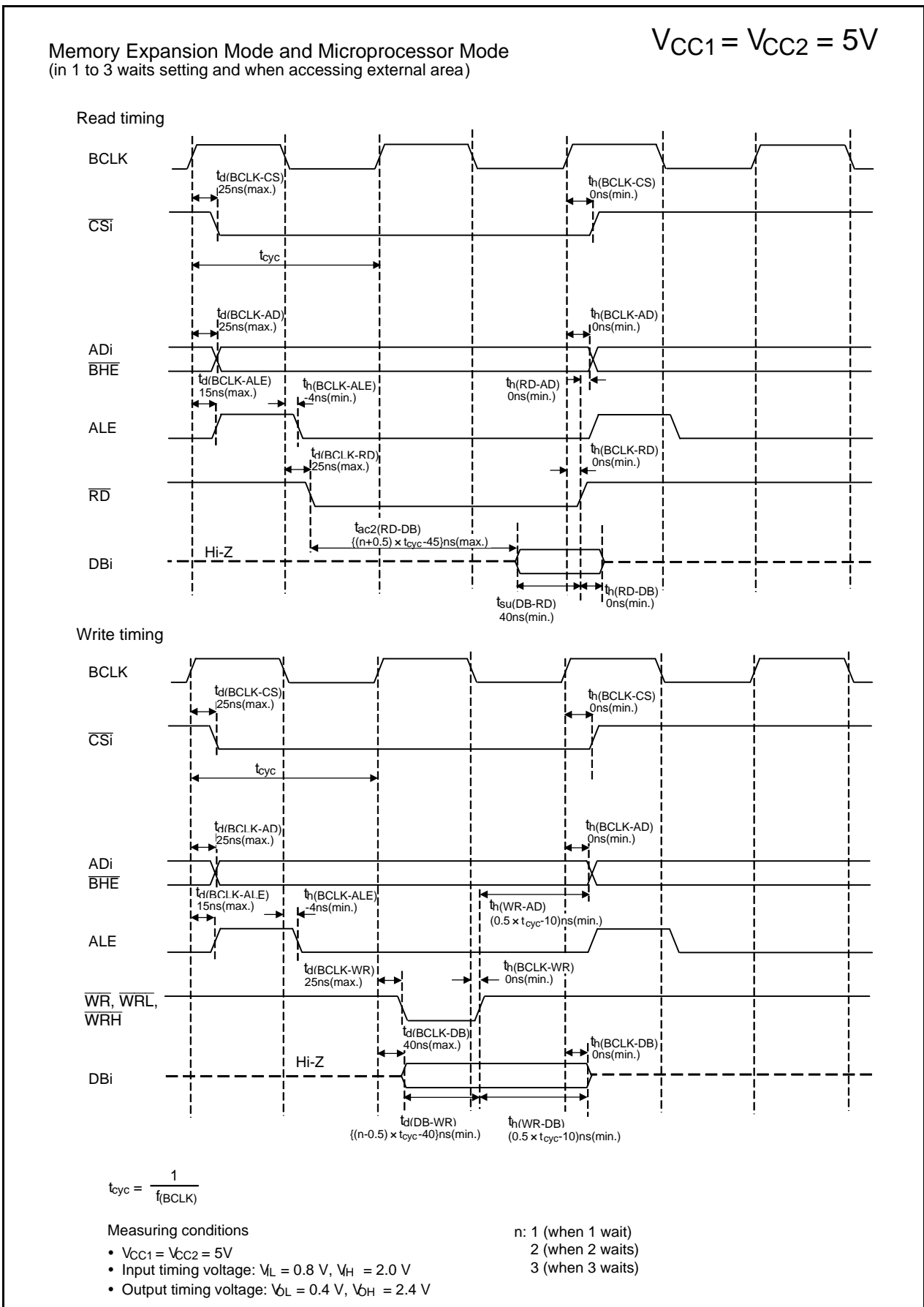
Figure 5.17 Timing Diagram
