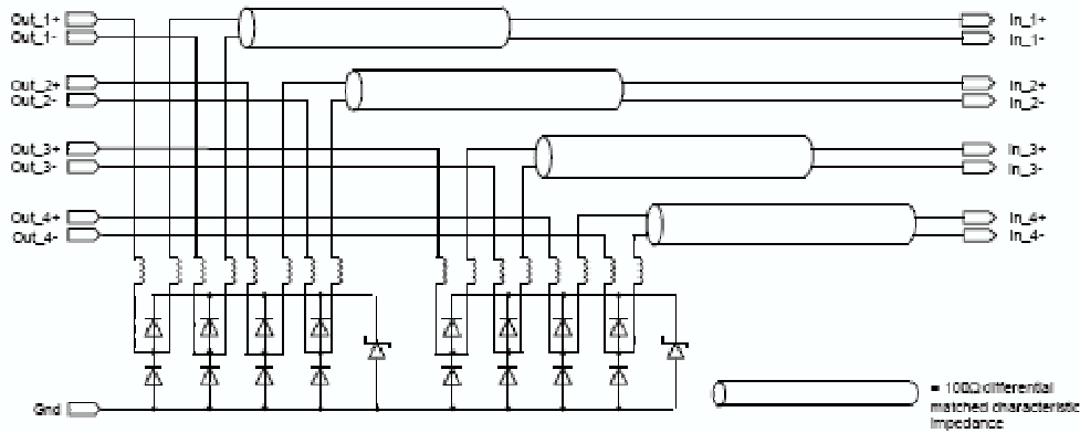
Figure 1. Block Diagram
