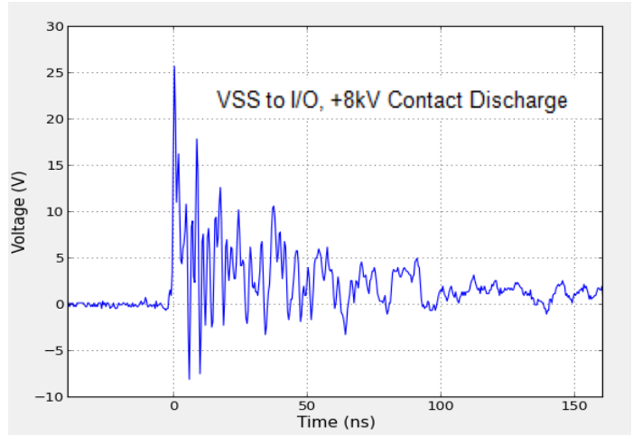
Figure 4. ESD response ESD response to IEC 61000-4-2
