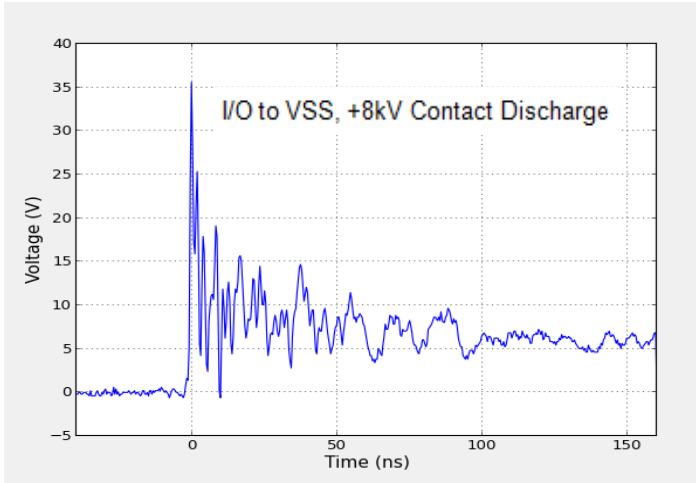
Figure 3. ESD response ESD response to IEC 61000-4-2
