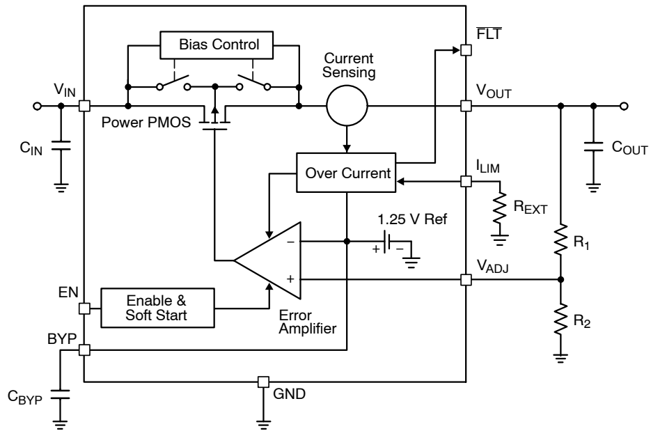
Figure 2. CAT6202 Functional Block Diagram
