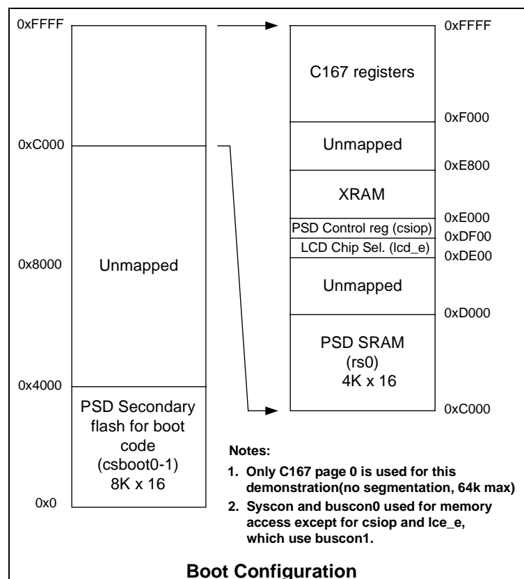
Figure 5—Memory Map: Simple C167CR/PSD4X35 Design
