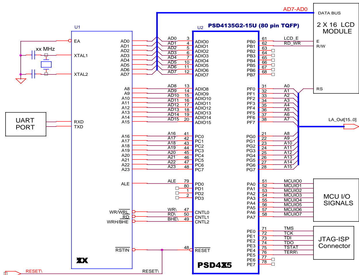
Figure 4 – Physical Connections, C167CR and PSD4X35
