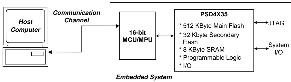
Figure 2 – Embedded flash system capable of IAP (2 devices)
