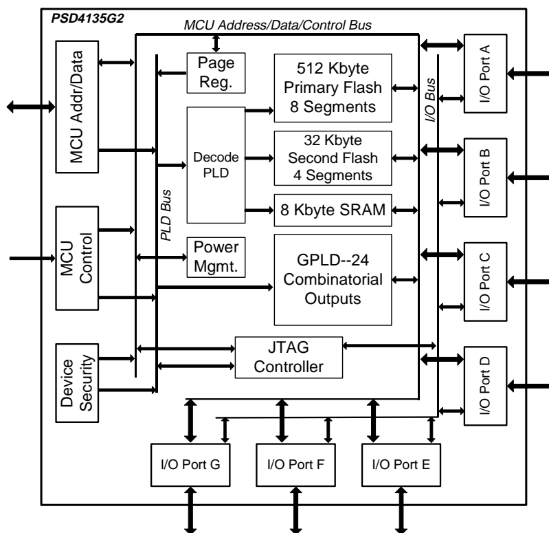
Figure 3—Top Level Block Diagram of PSD4X35
