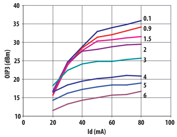
Figure 16. OIP3 vs Id and Frequency (GHz).
