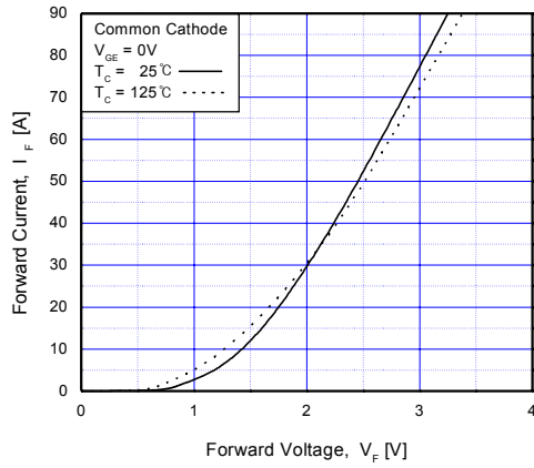
Fig 15. Forward Characteristics
