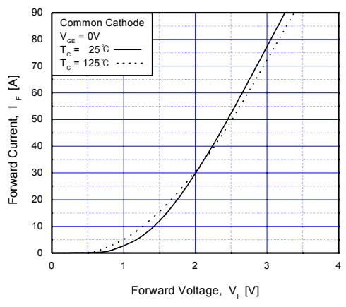
Fig 15. Forward Characteristics
