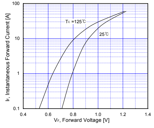
Fig 18. Rectifier ( Converter ) Characteristics
