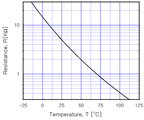
Fig 19. NTC Characteristics
