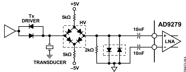
Figure 50. Input Overload Protection
