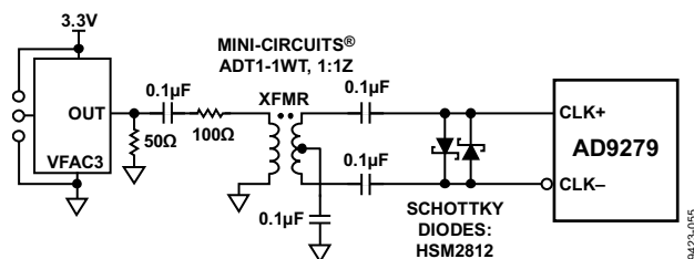
Figure 53. Transformer-Coupled Differential Clock
