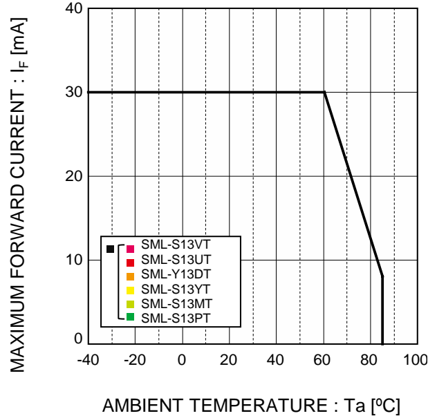
Fig.4 Derating
