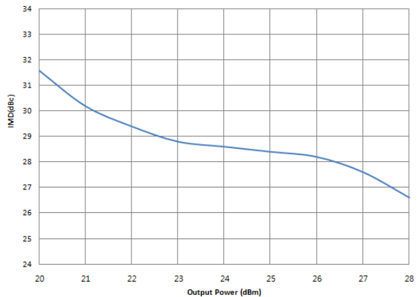
IMD vs Output Power Output power dBm per tone, 1 MHz spacing
