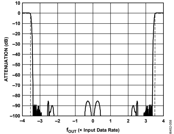
Figure 61. Interpolation/Modulation Combination of 4f_{DAC}/8 Filter
