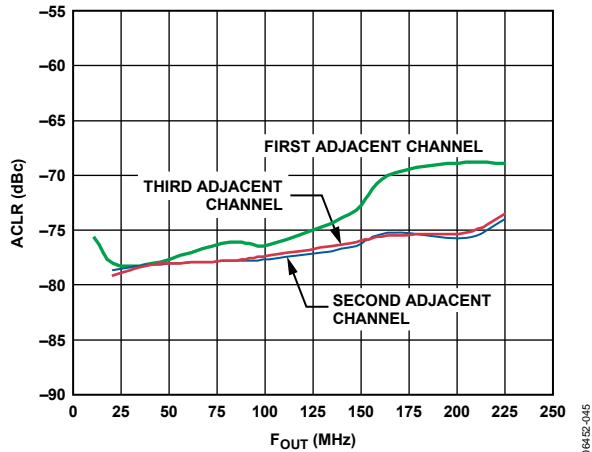
Figure 48. AD9776A ACLR vs. f_{OUT} , f_{DATA} = 122.88 MSPS, 4\times Interpolation, f_{DAC}/4 Modulation
