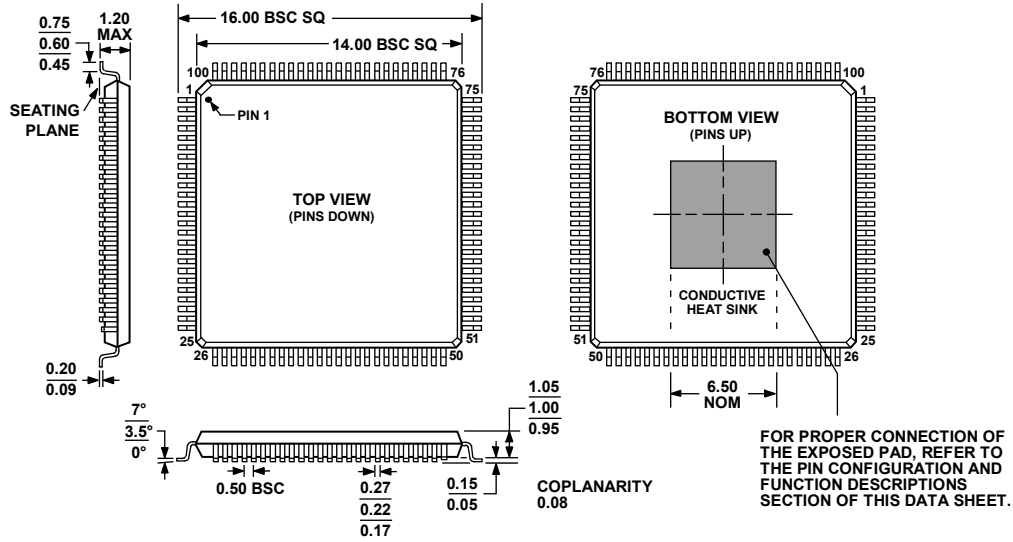
Figure 103. 100-Lead Thin Quad Flat Package, Exposed Pad [TQFP_EP] (SV-100-1)
