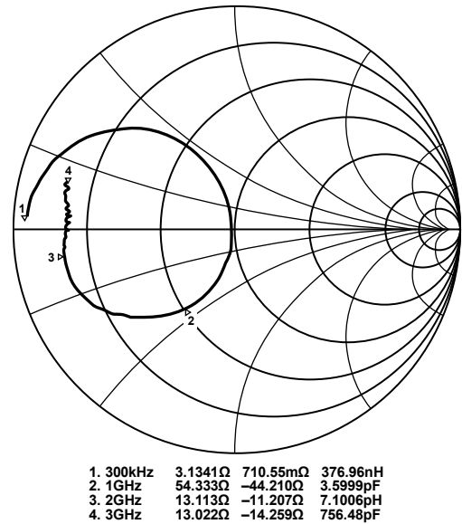
Figure 156. Measured Smith Chart Showing the DAC Output Impedance; f_{DAC} = 2.6 GSPS
