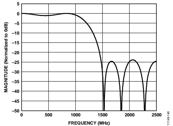
Figure 137. FIR25 2× Interpolation Filter Plot, Complete Frequency Response; f_{DAC} = 2.5 \text{ GHz}
