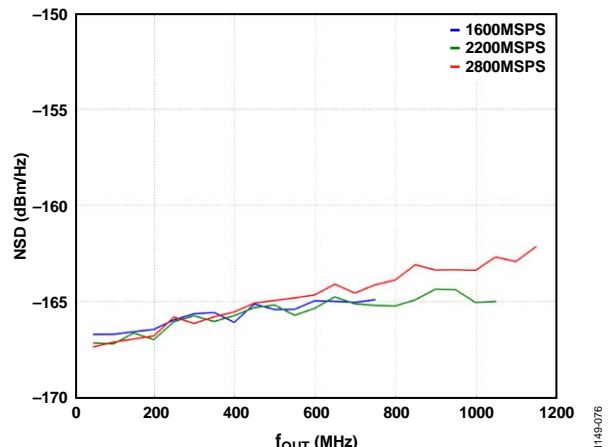
Figure 67. W-CDMA NSD vs. f_{OUT}
