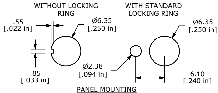
PANEL MOUNTING
