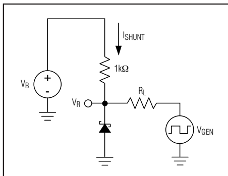
Figure 1. Load-Transient Test Circuit
