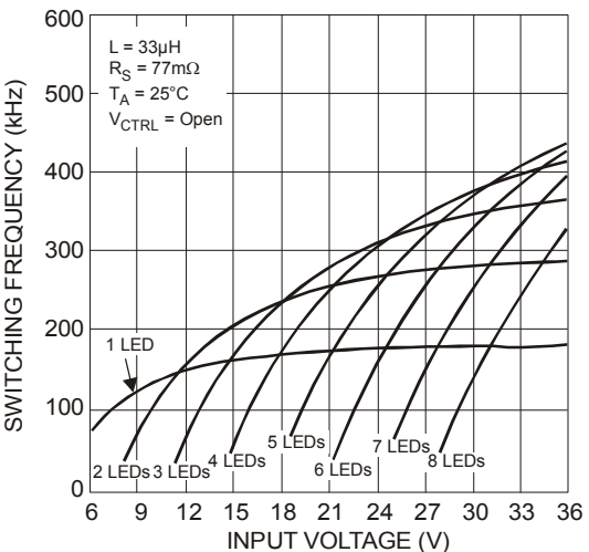
Figure 30. Switching Frequency vs. Input Voltage
