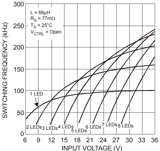
Figure 28. Switching Frequency vs. Input Voltage
