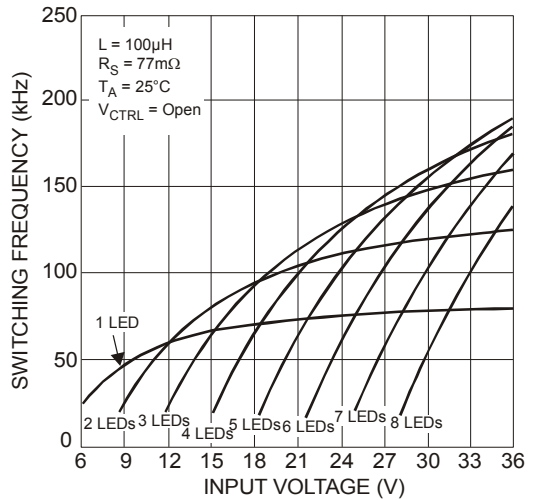
Figure 26. Switching Frequency vs. Input Voltage
