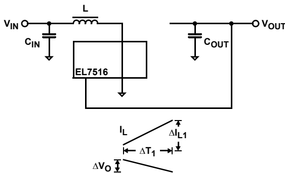
FIGURE 28. BOOST CONVERTER
