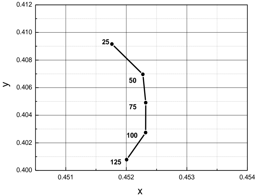
Fig 8. Chromaticity Coordinate vs. Junction Temperature I_F=30mA (2600K~3700K)
