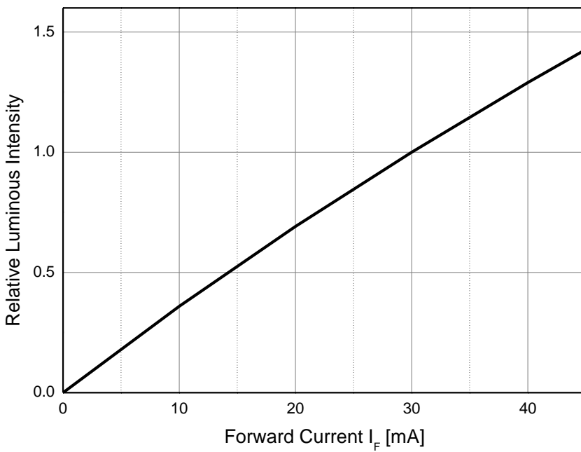
Fig 4. Forward Current vs. Relative Luminous Flux, T_a=25^\circ\text{C}
