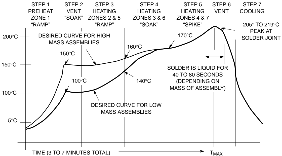
Figure 16. Typical Solder Heating Profile
