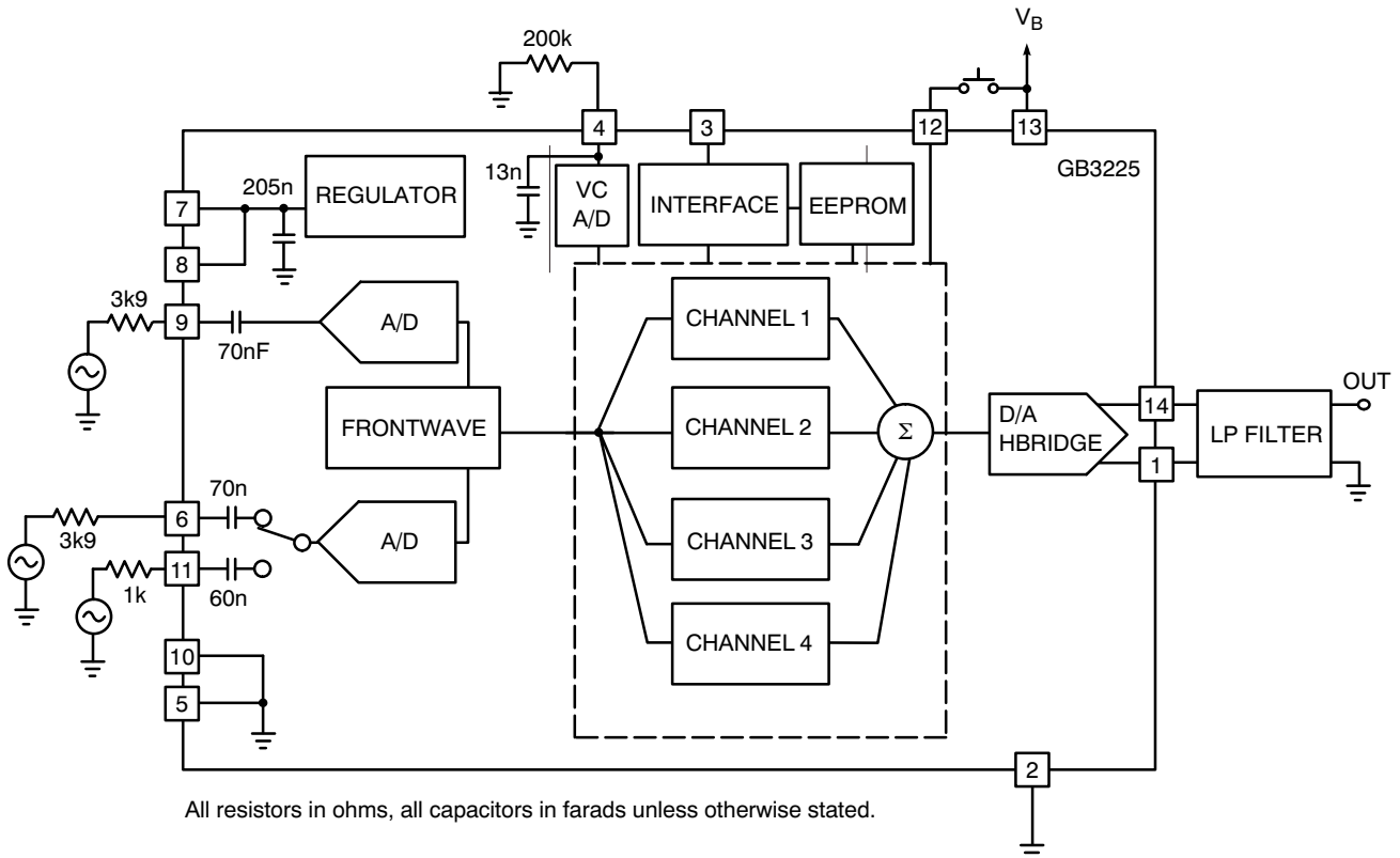
Figure 2. Test Circuit
