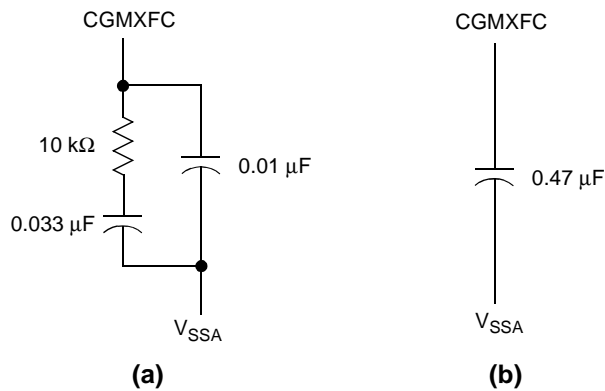
Figure 8-10. PLL Filter
