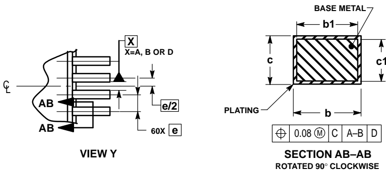
Figure 24-2. 64-Pin Low-Profile Quad Flat Pack (Case No. 840F)
