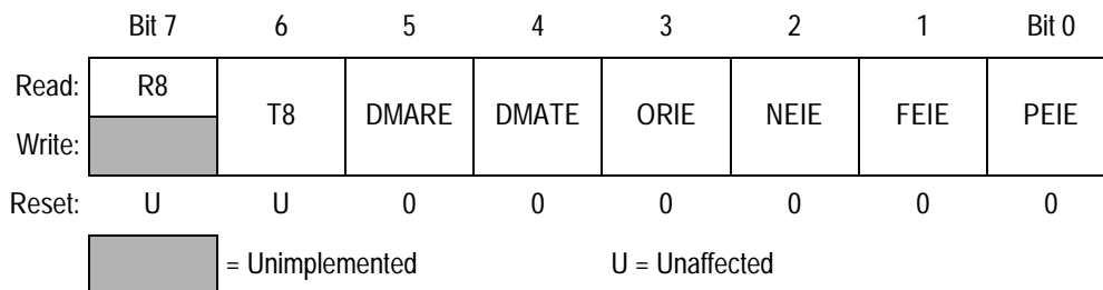
Figure 13-14. SCI Control Register 3 (SCC3)
