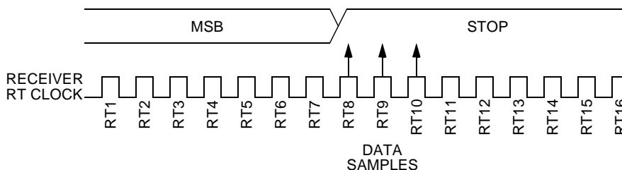
Figure 13-10. Slow Data
