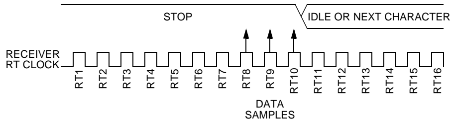
Figure 13-11. Fast Data
