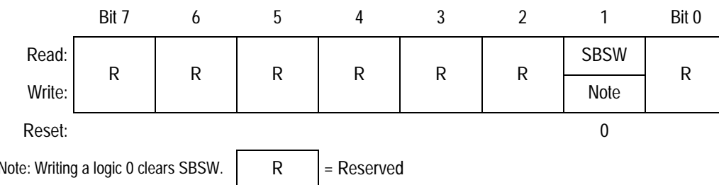
Figure 22-6. SIM Break Status Register (SBSR)
