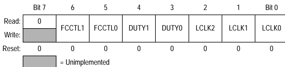
Figure 16-17. LCD Clock Register (LCDCLK)
