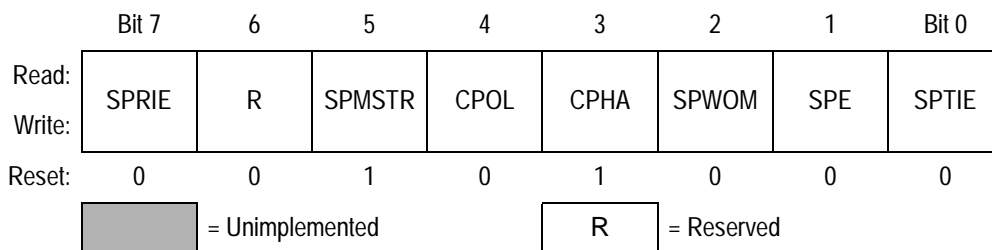
Figure 14-13. SPI Control Register (SPCR)
