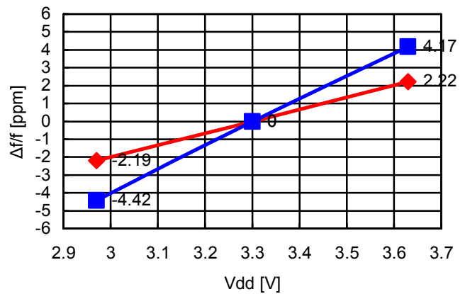
fcenter=20MHz, Vdd=3.3V±10%
