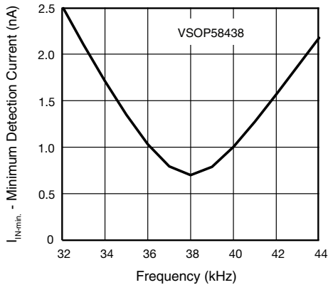
Fig. 4 - Bandpassfilter Characteristic
