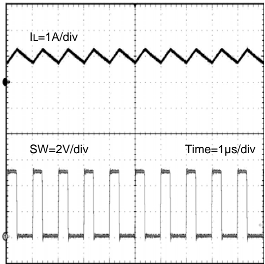
Figure 35. Switching Waveform (VIN = 5.0V, VOUT = 1.8V, IOUT = 1A, L=2.2µH)
