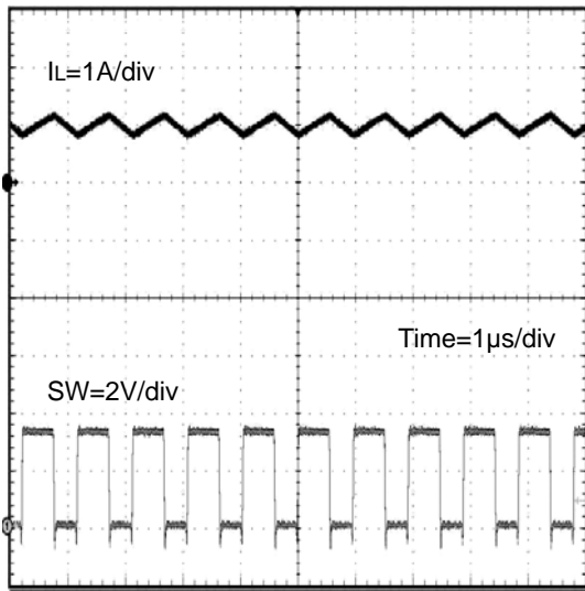
Figure 34. Switching Waveform (VIN = 3.3V, VOUT = 1.8V, IOUT = 1A, L=2.2µH)
