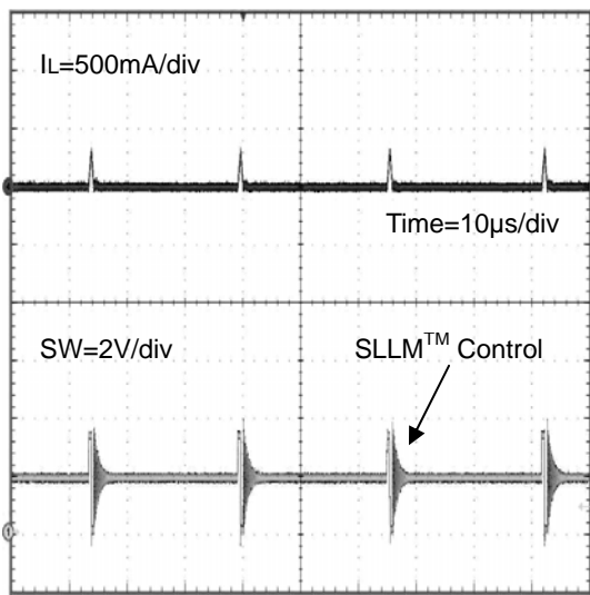
Figure 36. Switching Waveform with SLLM™ (VIN = 3.3V, VOUT = 1.8V, IOUT = 30mA, L=2.2µH)
