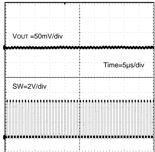
Figure 42. SW Waveform (PWM control) ( V_{IN} = 5.0\text{V} , V_{OUT} = 1.8\text{V} , I_{OUT} = 1\text{A} )
