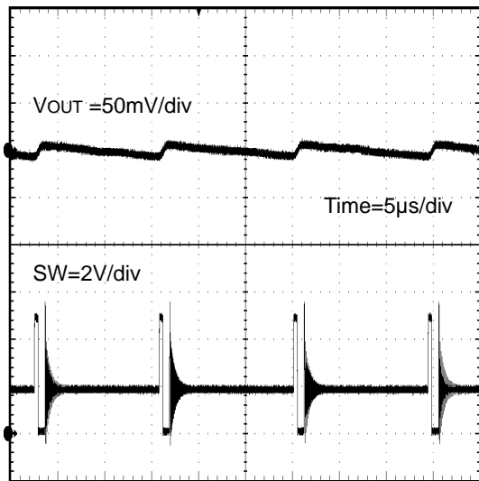
Figure 41. SW Waveform (SLLM™ control) ( V_{IN} = 5.0\text{V} , V_{OUT} = 1.8\text{V} , I_{OUT} = 50\text{mA} )
