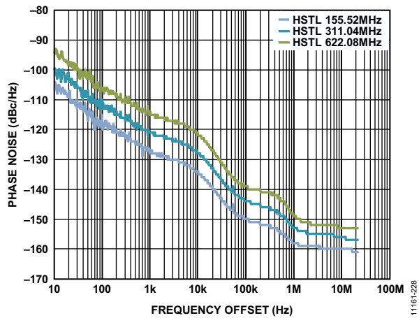
Figure 26. Absolute Phase Noise in HSTL with Clock Input at 622.08 MHz and Outputs = 622.08 MHz, 311.04 MHz, 155.52 MHz
