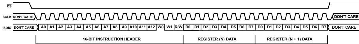
Figure 52. Serial Control Port Write—LSB First, 16-Bit Instruction, Two Bytes of Data
