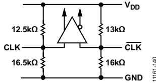
Figure 42. AD9508 Differential Input Stage
