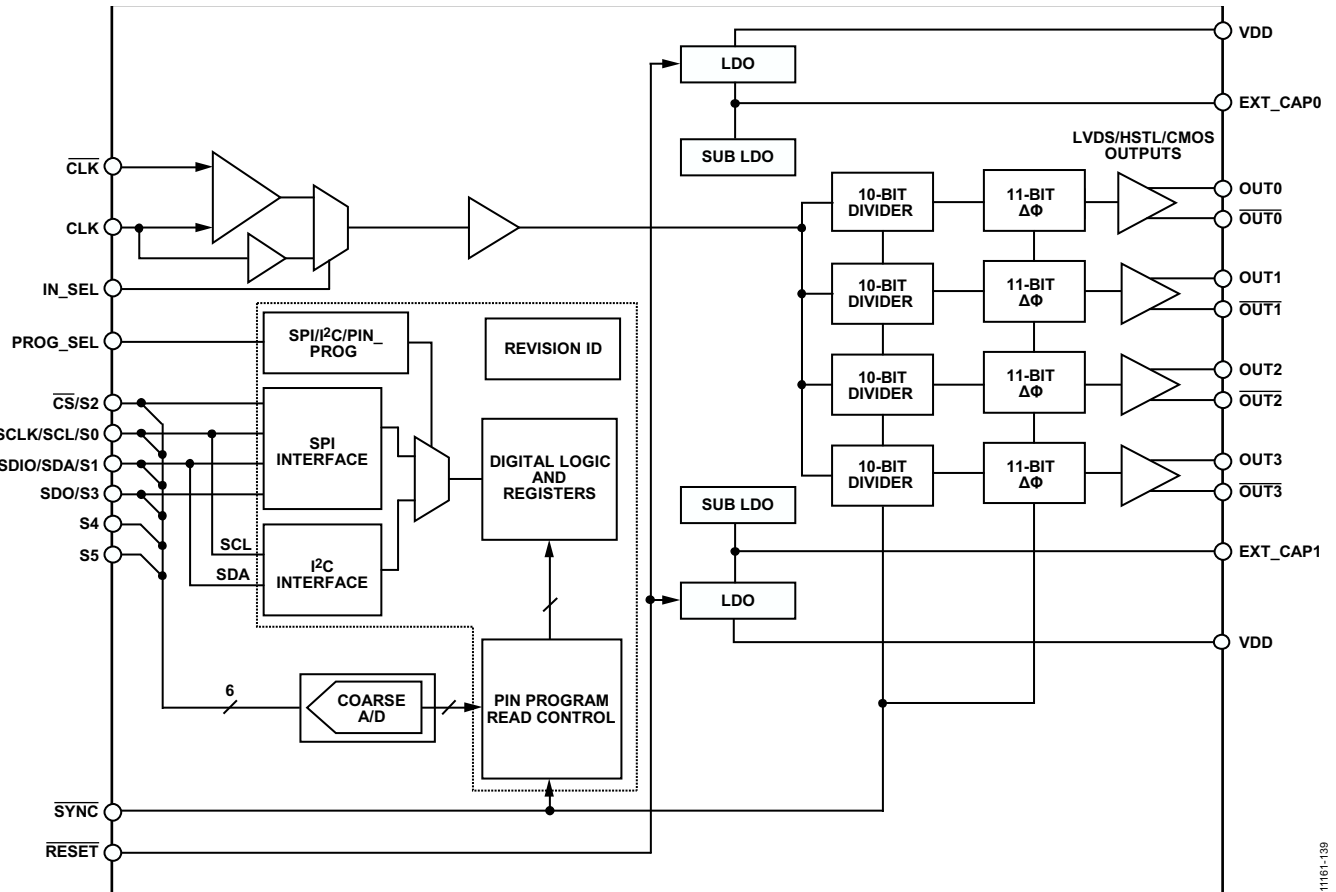
Figure 41. Detailed Block Diagram
