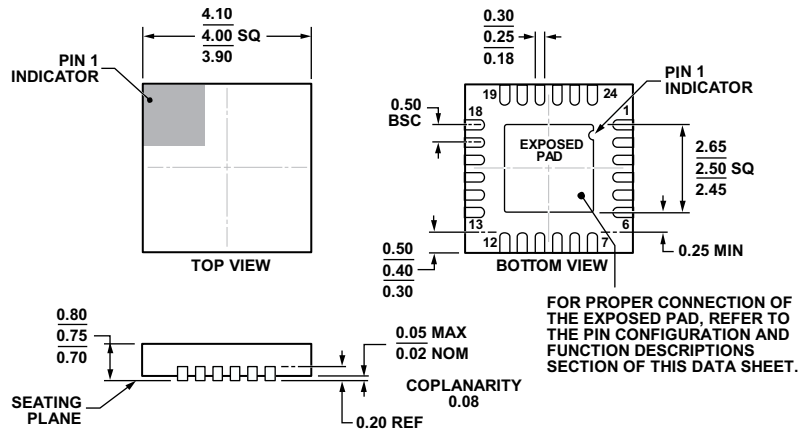
COMPLIANT TO JEDEC STANDARDS MO-220-WGGD. Figure 60. 24-Lead Lead Frame Chip Scale Package [LFCS P _WQ] 4 mm × 4 mm Body, Very Thin Quad (CP-24-7) Dimensions shown in millimeters
