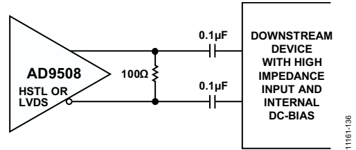
Figure 38. AC-Coupled LVDS or HSTL Output Driver (100Ω Resistor Can Go on Either Side of Decoupling Capacitors Placed As Close As Possible To The Destination Receiver)
