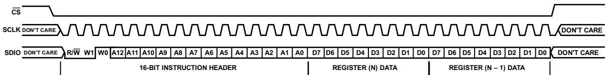
Figure 48. Serial Control Port Write—MSB First, 16-Bit Instruction, Two Bytes of Data
