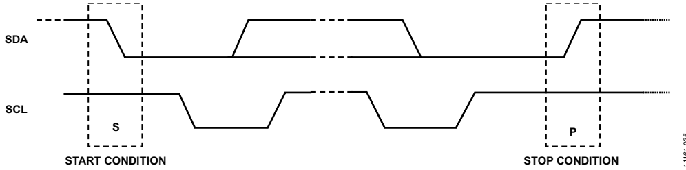
Figure 55. Start and Stop Conditions
