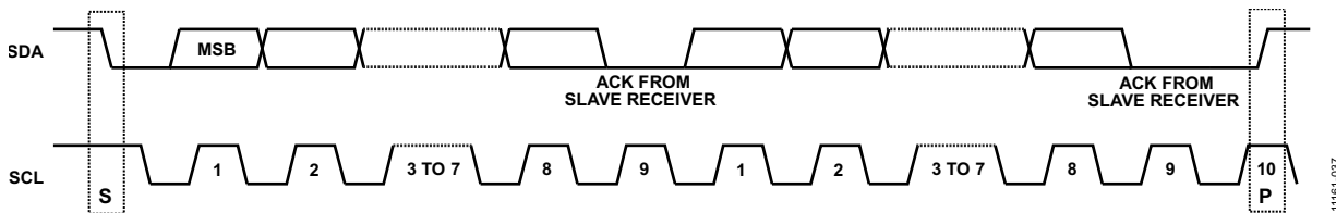
Figure 57. Data Transfer Process (Master Write Mode, Two-Byte Transfer)
