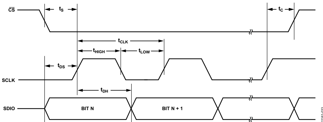
Figure 53. Serial Control Port Timing—Write
