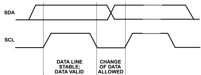
Figure 54. Valid Bit Transfer
