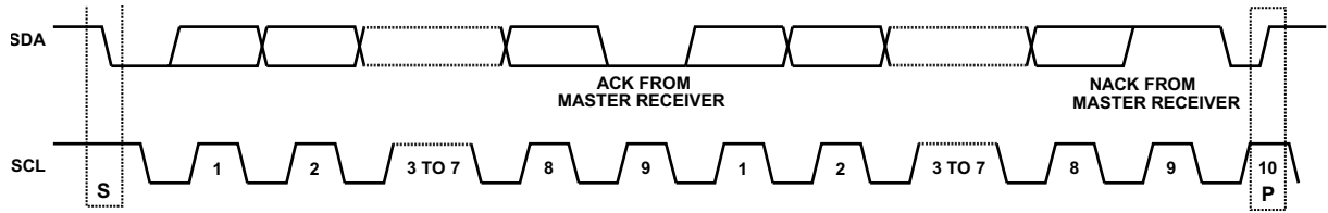
Figure 58. Data Transfer Process (Master Read Mode, Two-Byte Transfer)
