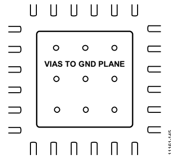
Figure 47. PCB Land Example for Attaching Exposed Paddle
