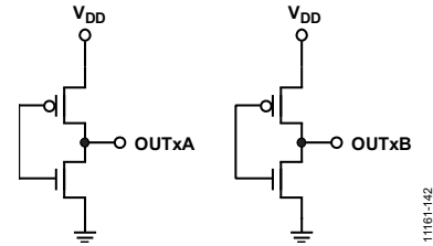
Figure 44. CMOS Equivalent Output Circuit
