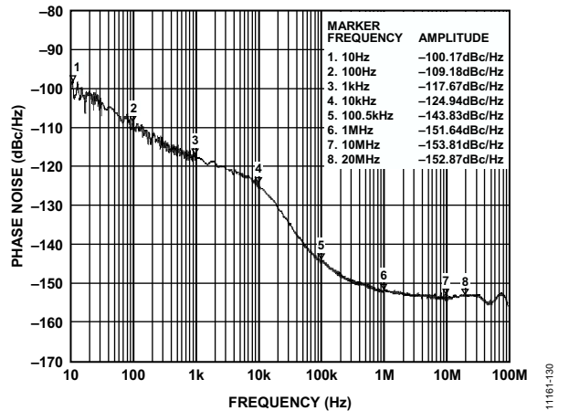
Figure 32. Additive Phase Noise with Clock Input = 622.08 MHz with LVDS Outputs = 622.08 MHz
