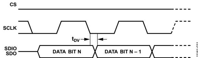
Figure 51. Timing Diagram for Serial Control Port Register Read
