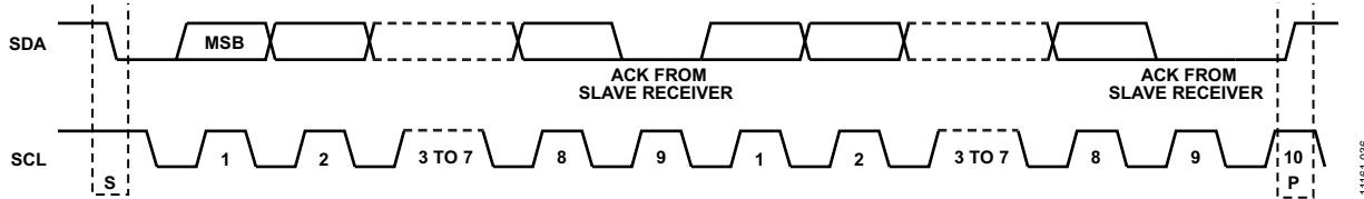
Figure 56. Acknowledge Bit
