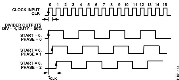
Figure 46. Phase Offset—All Dividers Set for DIV = 4, Phase Set from 0 to 2
