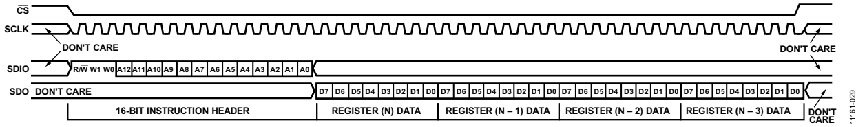
Figure 49. Serial Control Port Read—MSB First, 16-Bit Instruction, Four Bytes of Data
