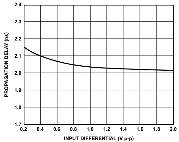
Figure 8. LVDS Propagation Delay vs. Input Differential Voltage
