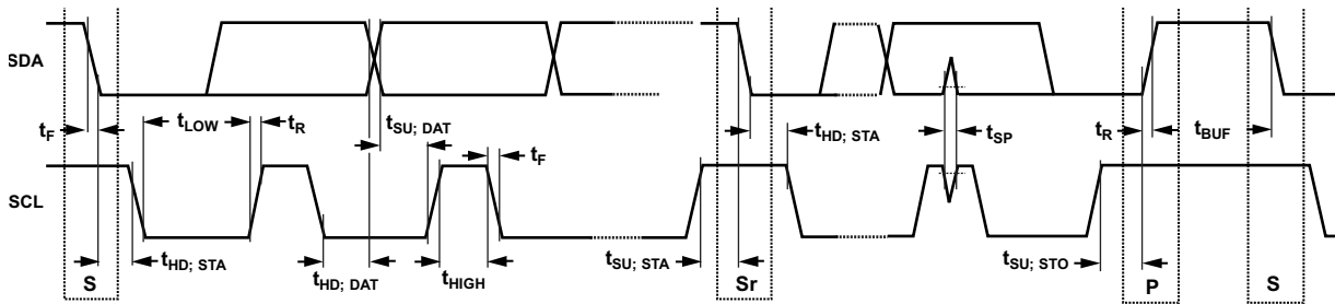
Figure 59. I 2 C Serial Port Timing
