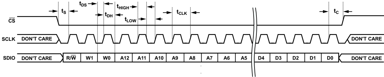
Figure 50. Serial Control Port Write—MSB First, 16-Bit Instruction, Timing Measurements
