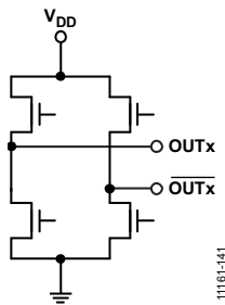
Figure 43. LVDS/HSTL Output Simplified Equivalent Circuit
