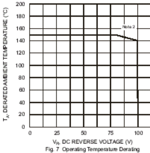
Fig. 7 Operating Temperature Derating
