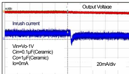
Inrush Peak Current=20mA( C_s=0.0047\mu F )
