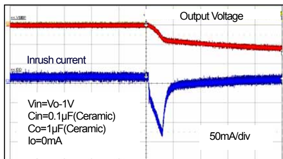
Inrush Peak Current=150mA( C_s =Open)
