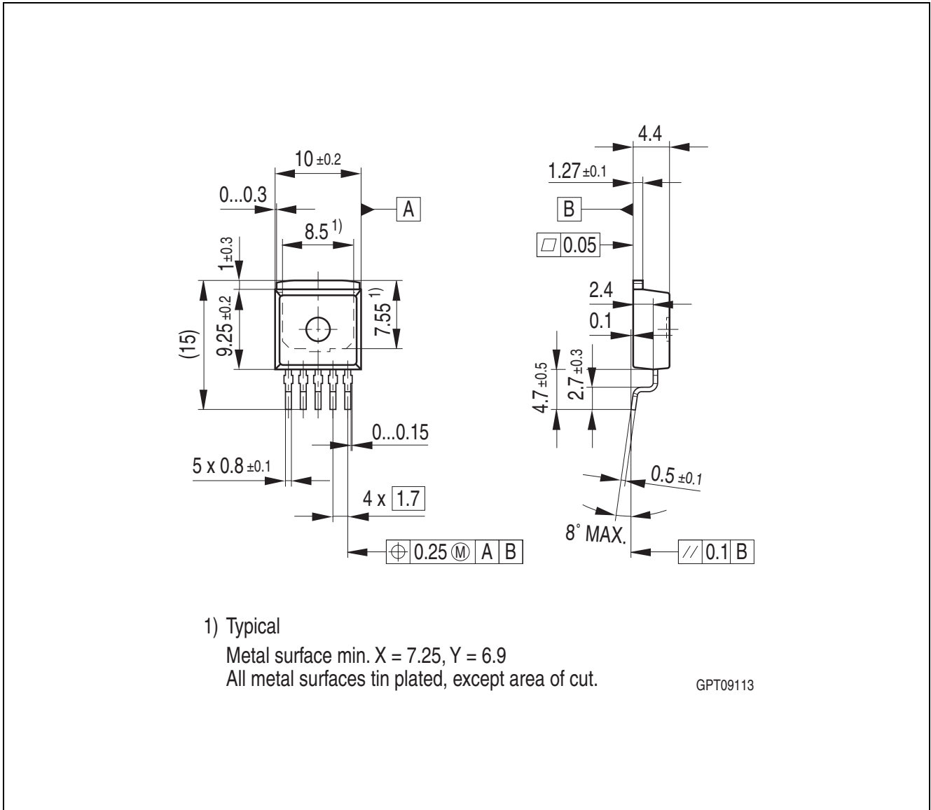
Figure 8 PG-TO263-5
