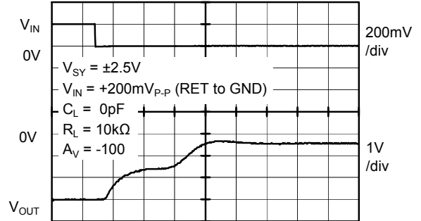
Time (20µs/div)
