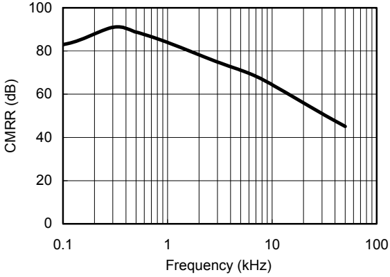
CMRR vs. Frequency at +5V
