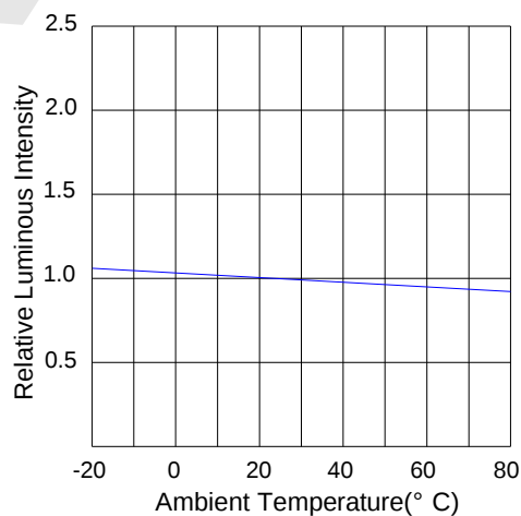
Relative Luminous Intensity VS. Ambient Temperature
