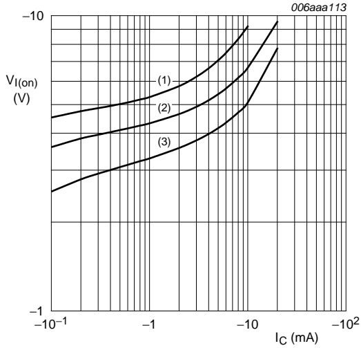
V_{CE} = -0.3 V (1) T_{amb} = -40^\circ C (2) T_{amb} = 25^\circ C (3) T_{amb} = 100^\circ C
