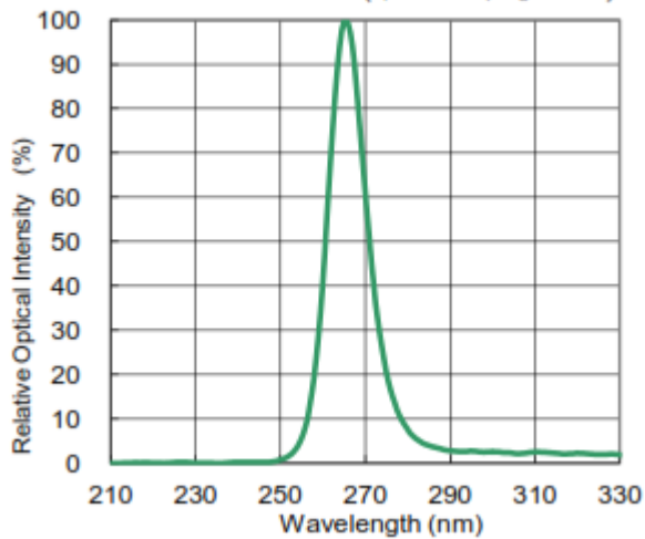
( I_F = 20\text{mA} , T_a = 25^\circ\text{C} )
