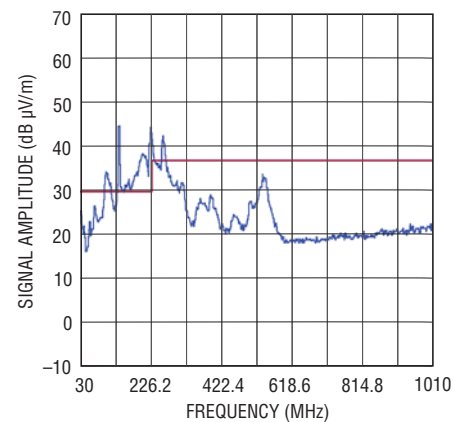
Figure 26. Radiated Emissions Scan of the LTM4676A Producing 1V OUT at 26A, from 12V IN . DC1811B-B Hardware with Outputs Paralleled. No Snubbers Applied. f_{SW} = 350 kHz. Measured in a 10m Chamber. Peak Detect Method
