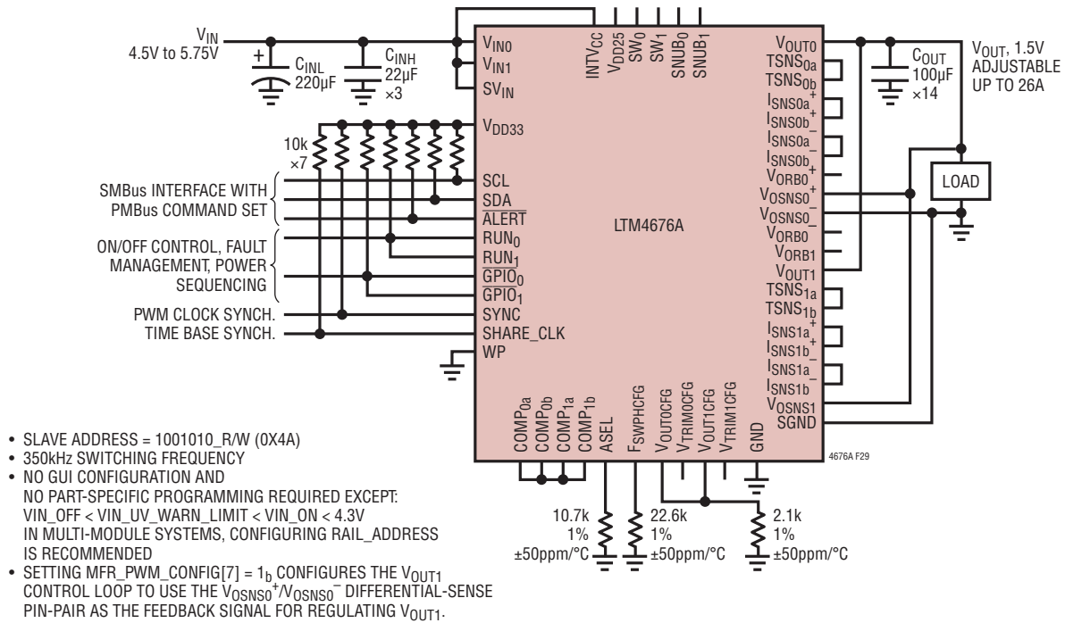
Figure 29. 26A, 1.5V Output DC/DC μModule Regulator with I 2 C/SMBus/PMBus Serial Interface
