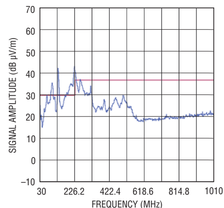
Figure 27. Radiated Emissions Scan of the LTM4676A Producing 1V OUT at 26A, from 12V IN . DC1811B-B Hardware with Outputs Paralleled. 1 \Omega (1/4W rated) Snubber Resistors Applied from SNUB_n to GND. f_{SW} = 350 kHz. Measured in a 10m Chamber. Peak Detect Method
