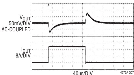
FIGURE 29 CIRCUIT AT 5\text{V}_{\text{IN}} , VOUT_COMMAND n SET TO 1.000V. 0A TO 20A LOAD STEP AT 20A/µs
