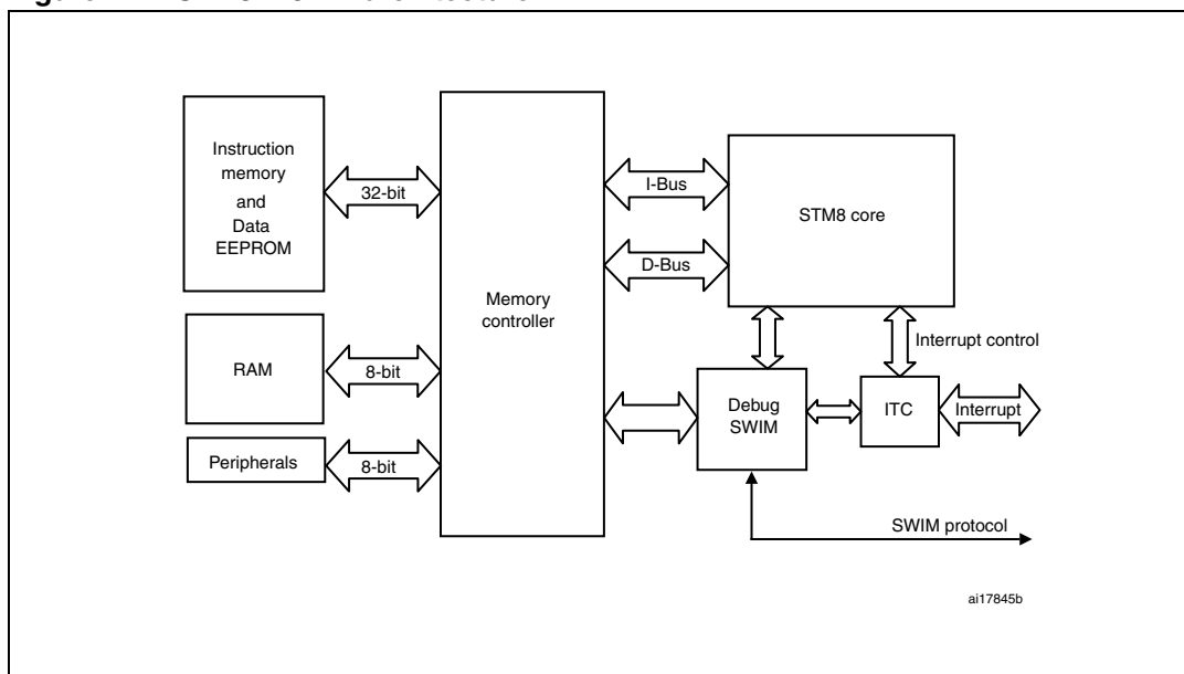
Figure 2. STM8TL5xxx architecture
