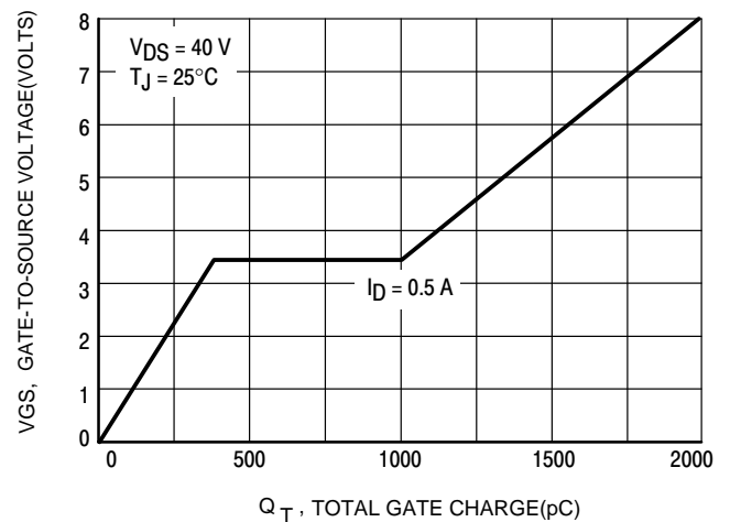
Figure 6. Gate Charge
