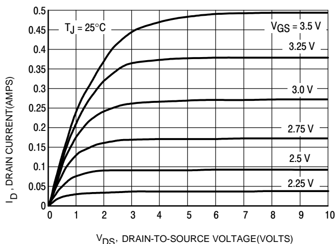
Figure 2. On-Region Characteristics
