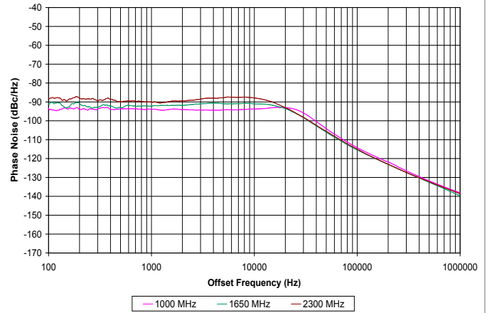
Phase Noise
