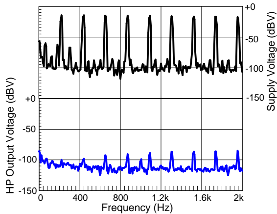
GSM Power Supply Rejection vs. Frequency
