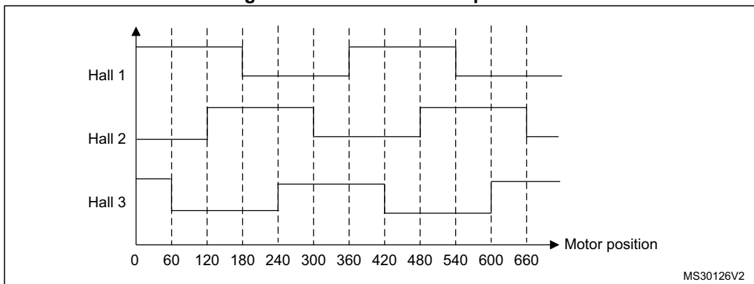
Figure 10. Commutation sequence
