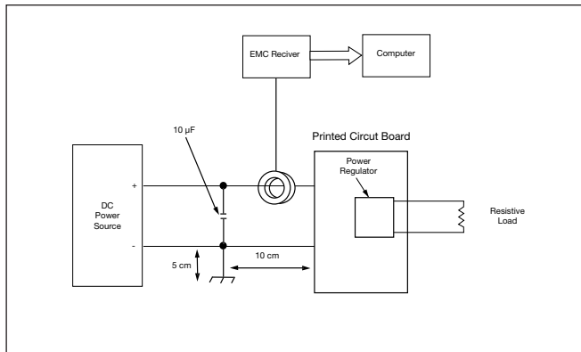
Test set up.
