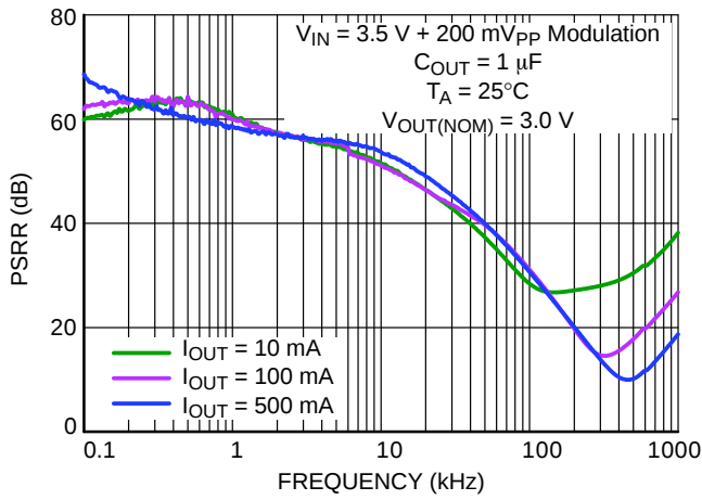
Figure 27. PSRR vs. Frequency & Output Current
