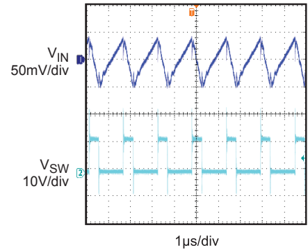
Input Ripple Voltage I_{OUT}=3A
