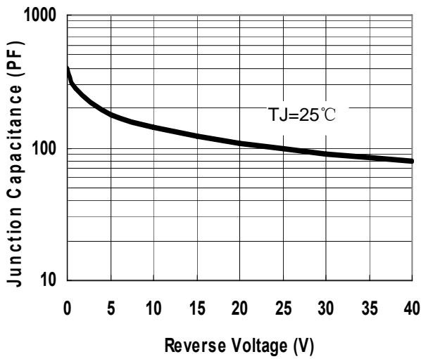
Fig.1-Typical Junction Capacitance
