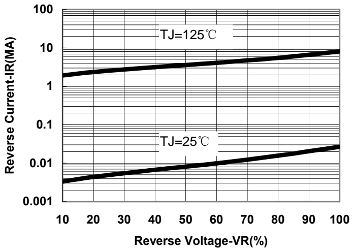
Fig.2-Typical Reverse Characteristics
