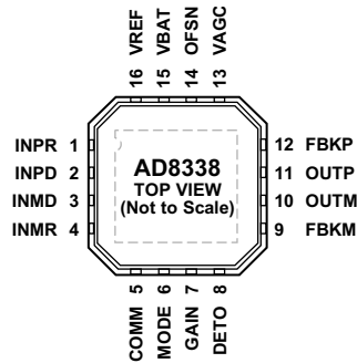
Figure 3. Pin Configuration
