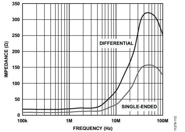
Figure 14. Output Impedance vs. Frequency
