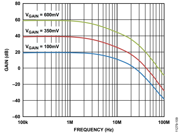
Figure 7. Gain vs. Frequency, R_{IN} = 50\ \Omega , 20 dB Steps
