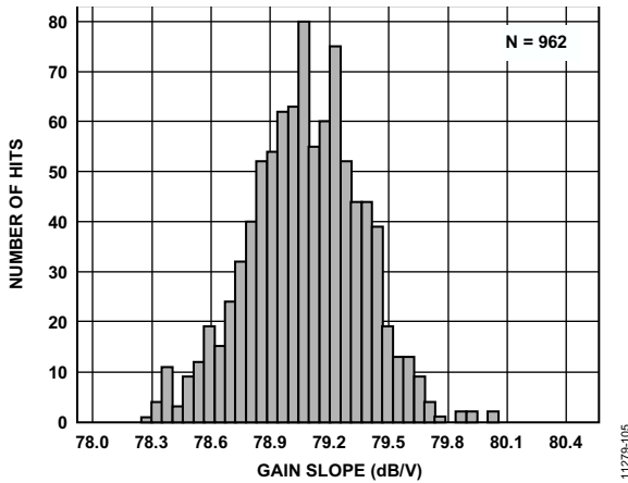
Figure 5. Gain Slope Histogram
