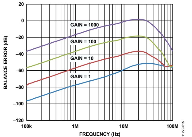
Figure 15. Output Balance Error vs. Frequency
