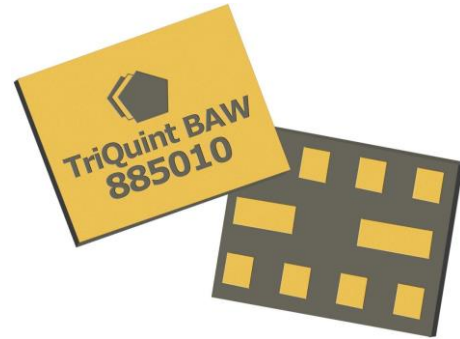
CSP-1713BT package: 1.7 x 1.3 x 0.46 mm
